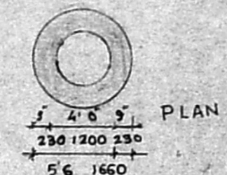
Well detail
