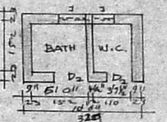
PLAN OF BATH & W.C.
