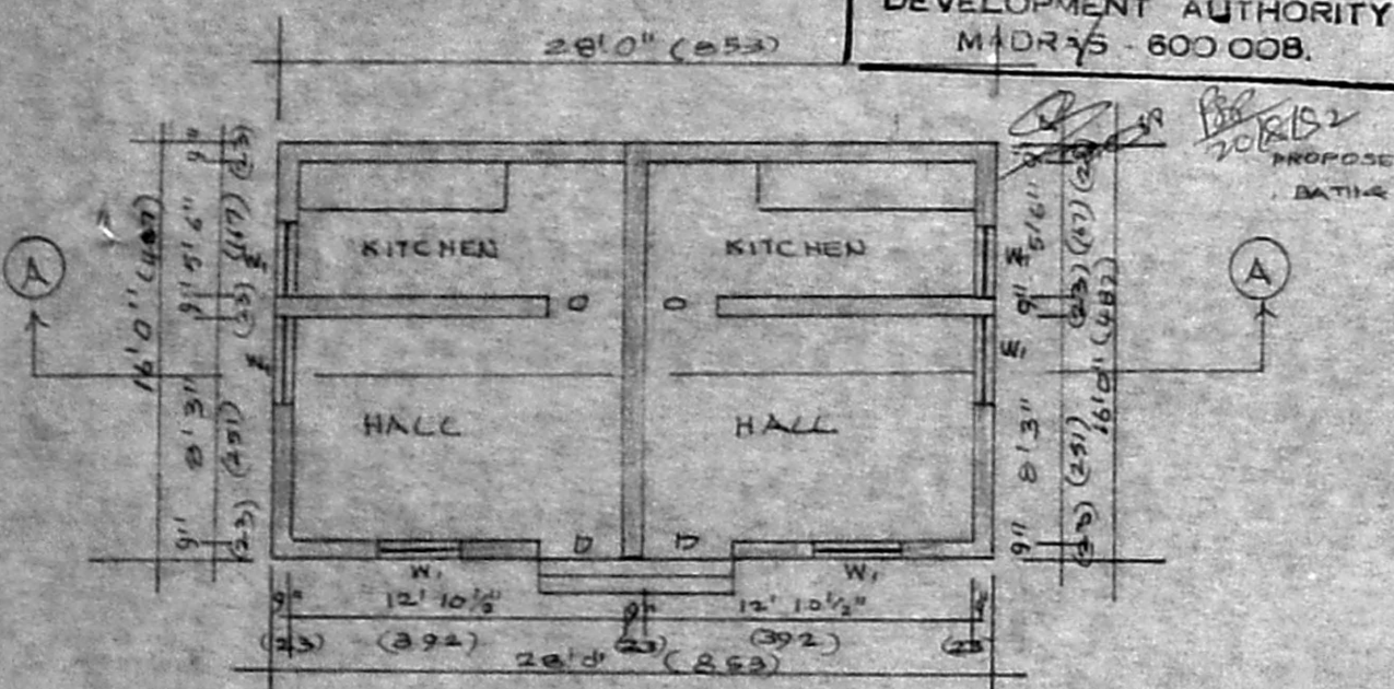
Proposed plan SCALE 1:100
